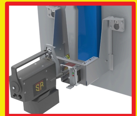
MDU WITH ATTACHED TAA PROPERLY ENGAGED WITH DRIVE RINGS AND LOCKING PIN, READY FOR SDB AND HHC COMMUNICATION CABLES
