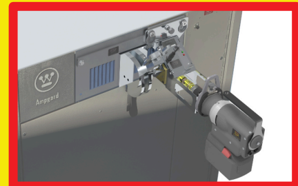
MDU WITH ATTACHED TAA PROPERLY ENGAGED WITH DRIVE RINGS AND LOCKING PIN, READY FOR SDB AND HHC COMMUNICATION CORDS
