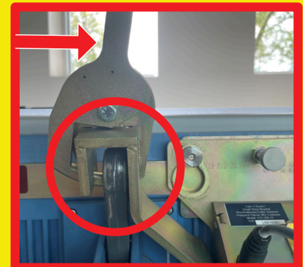
LEVER LATCH SECURED THROUGH HANDLE LOOP OF OPEN/CLOSE LEVER.
