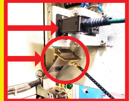
75R PLUG ENGAGED AND SDB CHAIN CORRECTLY PLACED OVER RACKING HANDLE IN CUBICLE
