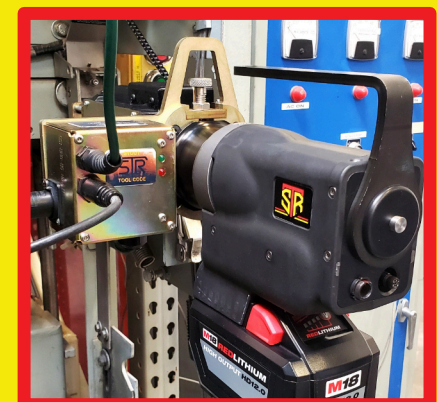
MDU PROPERLY ENGAGED WITH DRIVE RINGS AND LOCKING PIN, READY FOR SDB AND HHC COMMUNICATION CORDS
