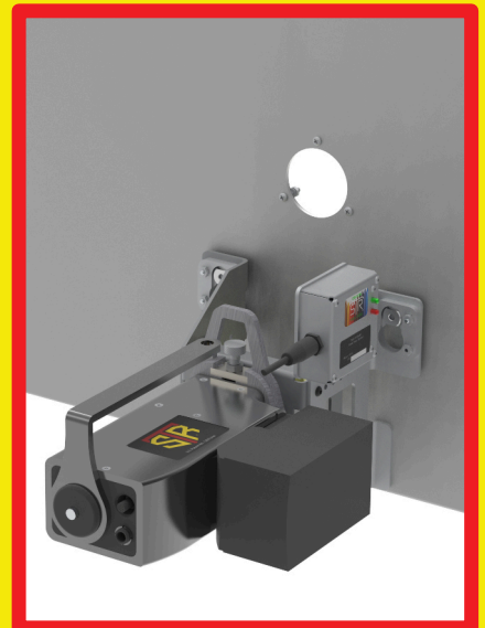
MDU AND TAA ENGAGED WITH RACKING PORT AND LOCKED INTO DRIVE RINGS, READY FOR COMMUNICATION CORDS FROM SDB AND HHC
