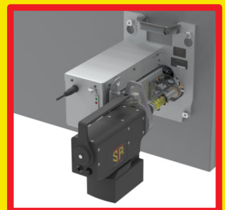
MDU WITH ATTACHED TAA PROPERLY ENGAGED WITH DRIVE RINGS AND LOCKING PIN, READY FOR SDB AND HHC COMMUNICATION CORDS
