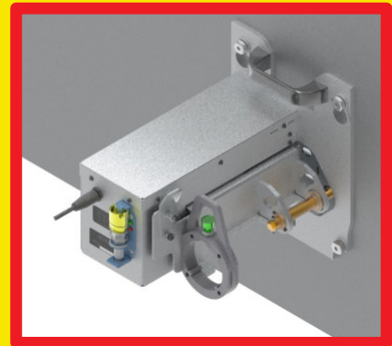
SDB SUSPENDED FROM CUBICLE FACE USING CUBICLE KIT SHOULDER NUTS
